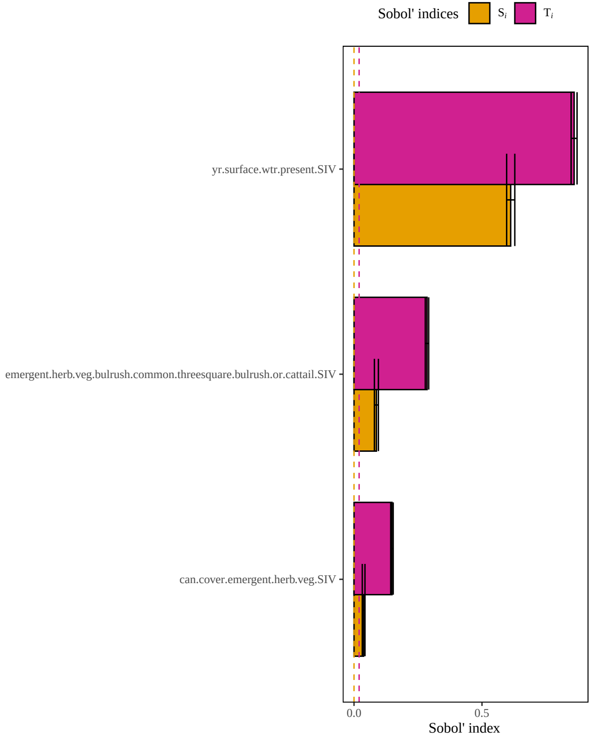
Figure 6. Results of a sensitivity analysis for the muskratHW model based on a limiting factor structure. Dashed lines represent baseline numerical approximation error for S_i and T_i ( i.e. , dummy variables).
