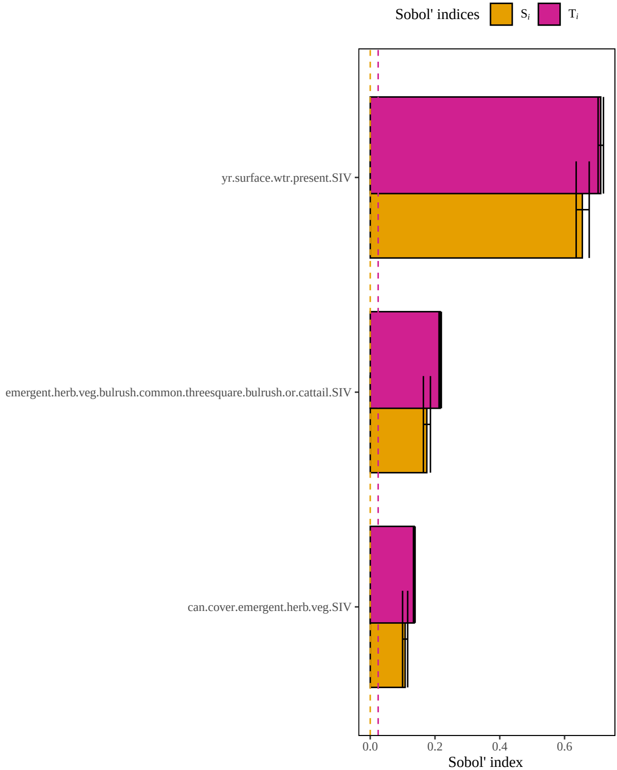
Figure 5. Results of a sensitivity analysis for the muskrathHW model based on a geometric mean structure. Dashed lines represent baseline numerical approximation error for S_i and T_i ( i.e. , dummy variables).
