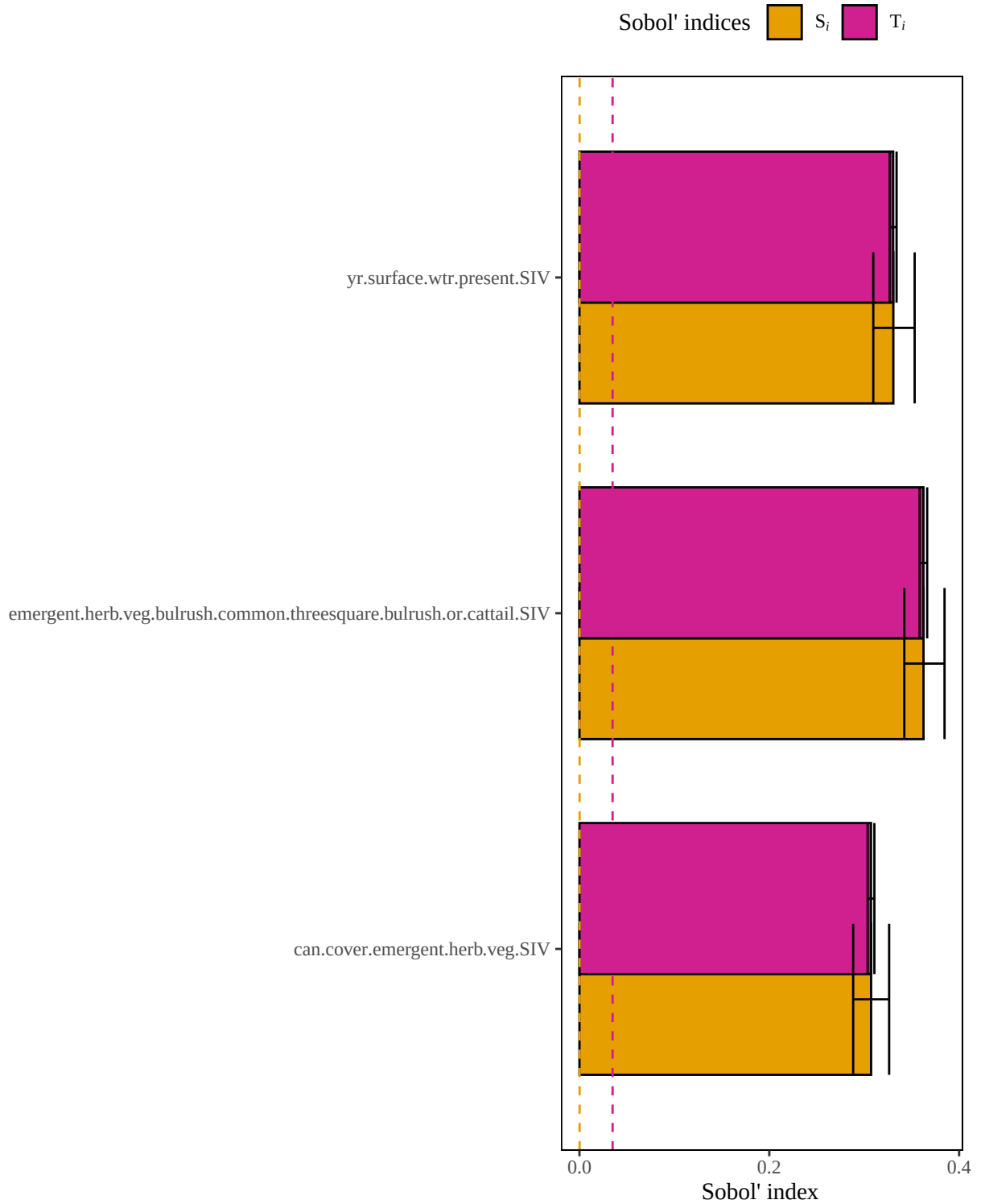
Figure 4. Results of a sensitivity analysis for the muskrathHW model based on an arithmetic mean structure. Dashed lines represent baseline numerical approximation error for S_i and T_i ( i.e. , dummy variables).
